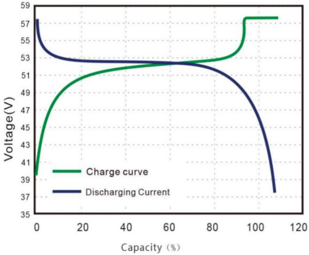
● Charge and discharge curve @0.5C 25°C
