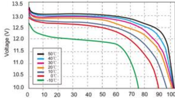
Different Temperature Discharge Curve
