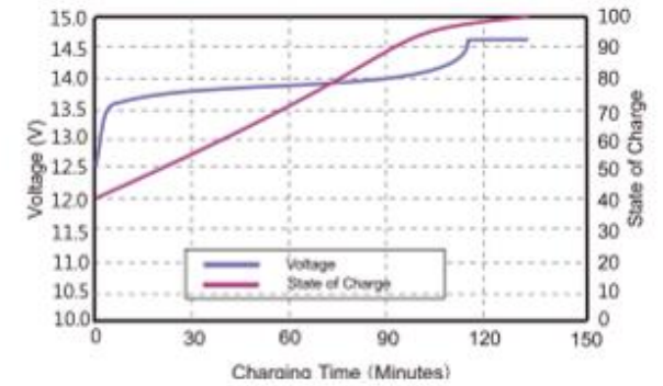
State of Charge Curve
