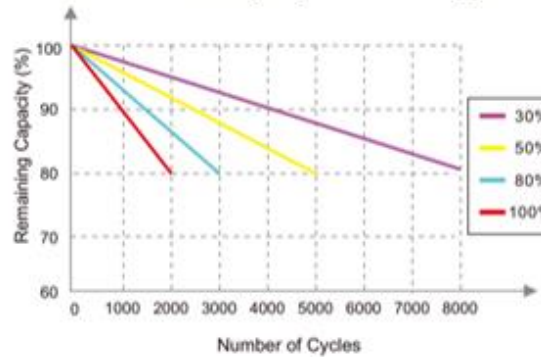
Cycle Life Curve
