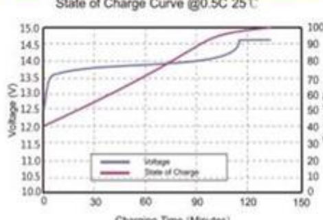
State of Charge Curve
